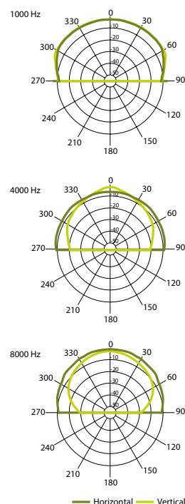
HORIZONTAL / VERTICAL POLAR DIAGRAMS
