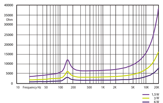
IMPEDANCE
